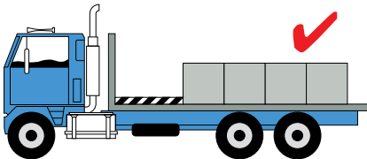
The headboard and extra blocking can be used to stop load shift.
