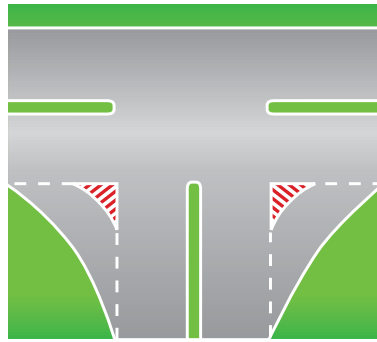
Fig. 3 – Traffic islands
